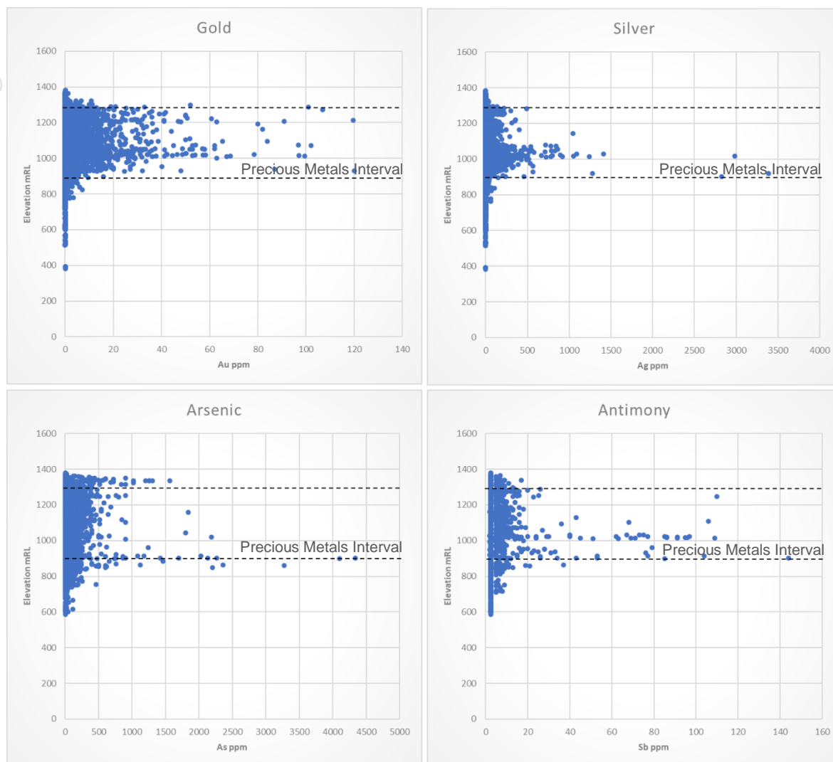
FIGURE 3: Charts showing vertical distribution of precious and pathfinder metals in drilling assay data at Way Lingo. High grade gold and silver are well defined as occurring between 1250 and 900 metres elevation. Arsenic is anomalous at the upper and lower parts of the precious metals interval and elevated antimony typically occurs near the base of the precious metals interval. The Maul Vein is exposed at an elevation of 1270 metres and is inferred to potentially lie immediately above the main precious metals interval.
