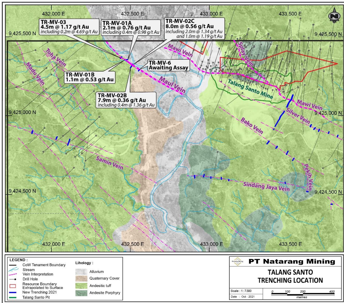
FIGURE 2: Map showing geology and trench locations at the Maul Vein target.
