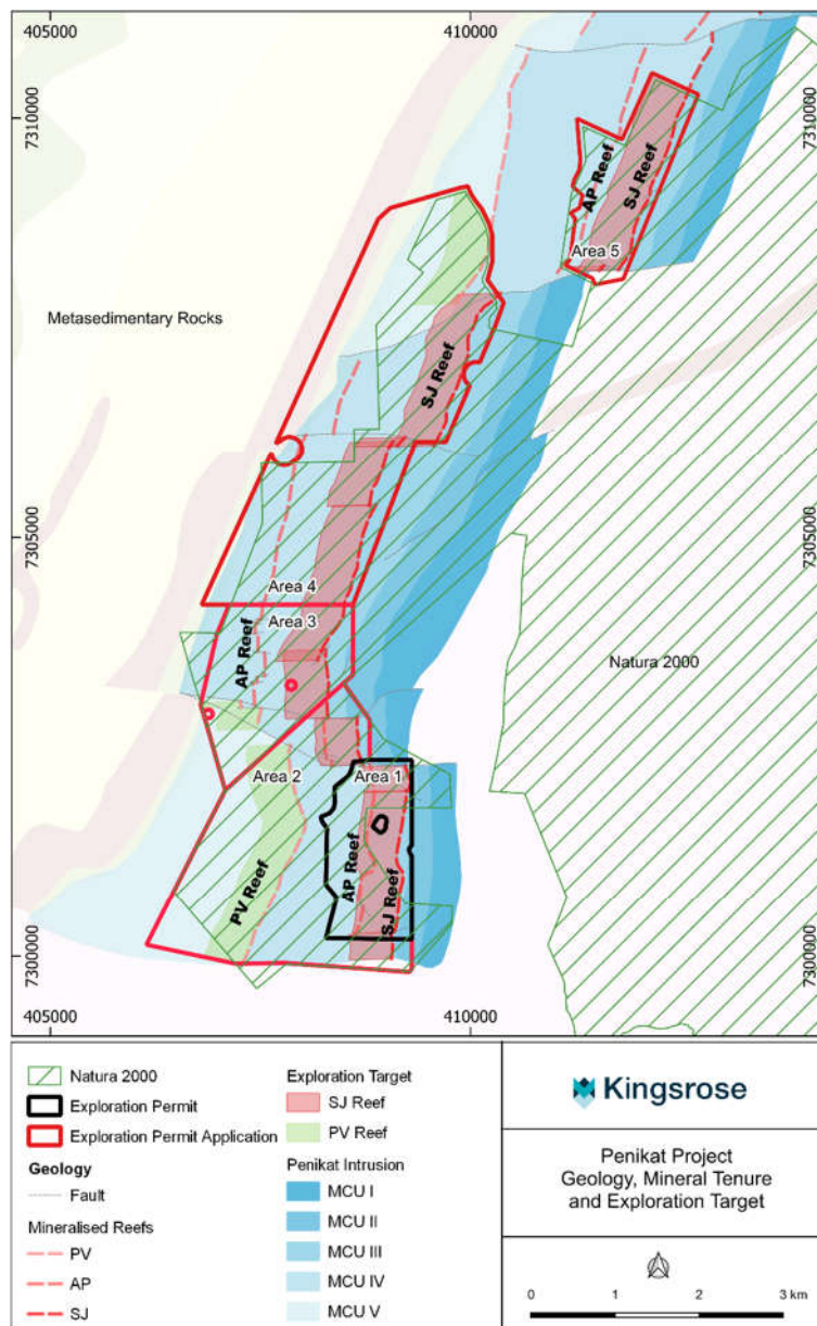
Figure 2: Penikat geology and Exploration Target announced 28 June 2022.
