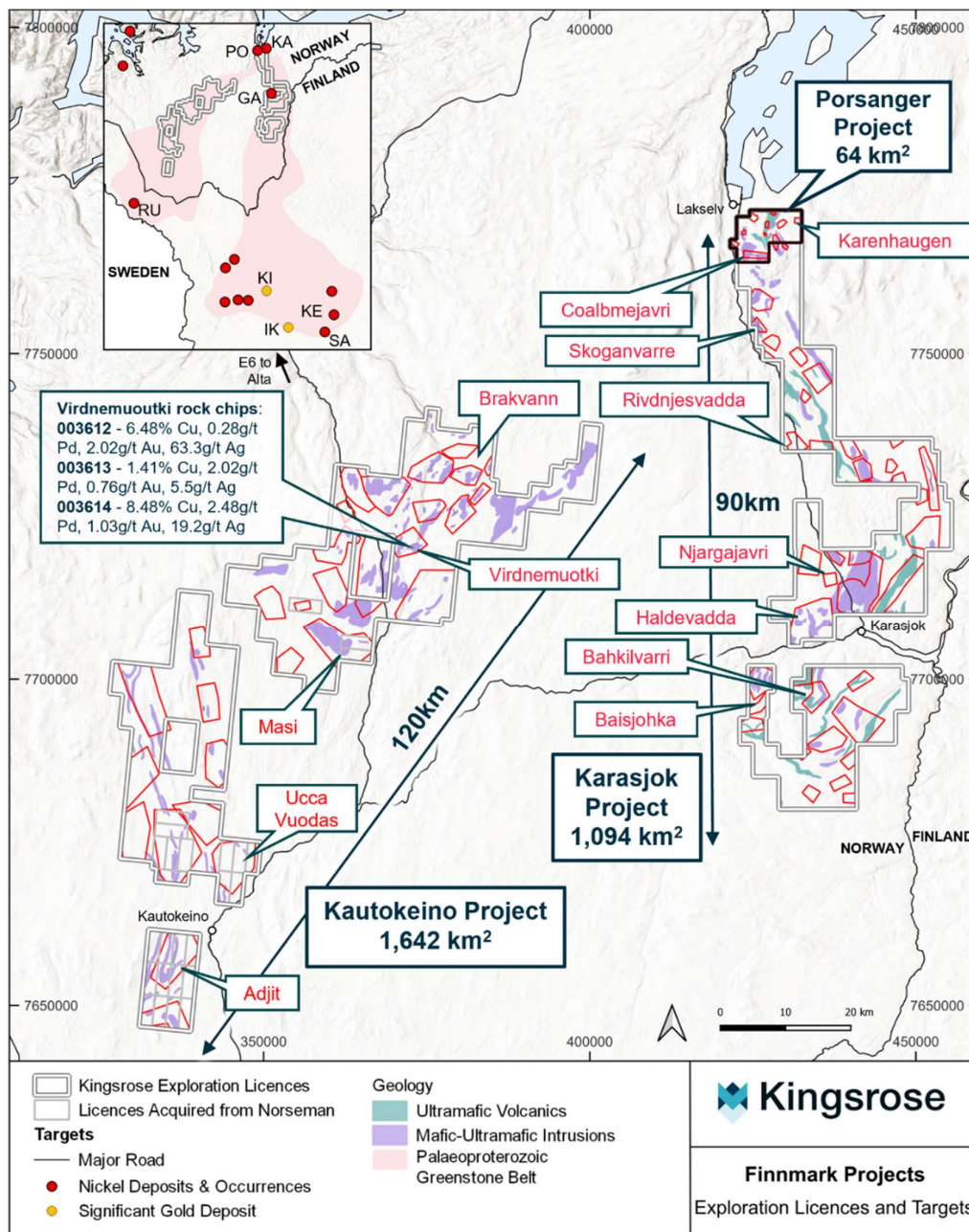
Figure 1: Location of the Porsanger project, and Karehaugen prospect, as well as Kingsrose exploration licences in the Karasjok and Kautokeino greenstone belts.
