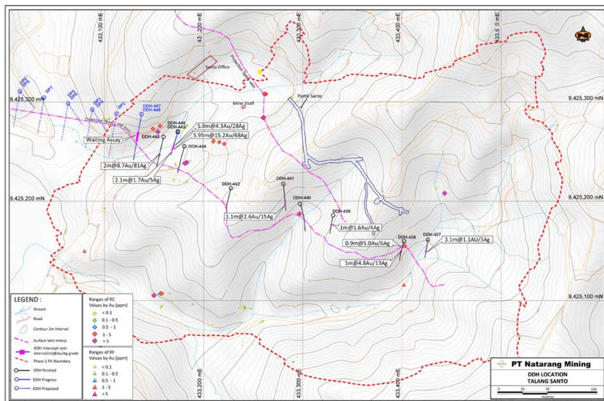
Figure 2 | Drill hole locations along the Talang Santo dilutinal vein swarm
